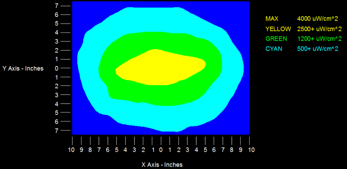
TOP INTENSITY PROFILE AT 15 IN (38 CM)
