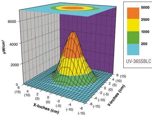
Surface Contour Profile at 15 in (38 cm)
